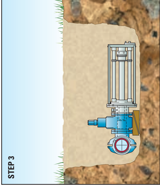
OPEN VALVE AND ACTIVATE TAPPING
